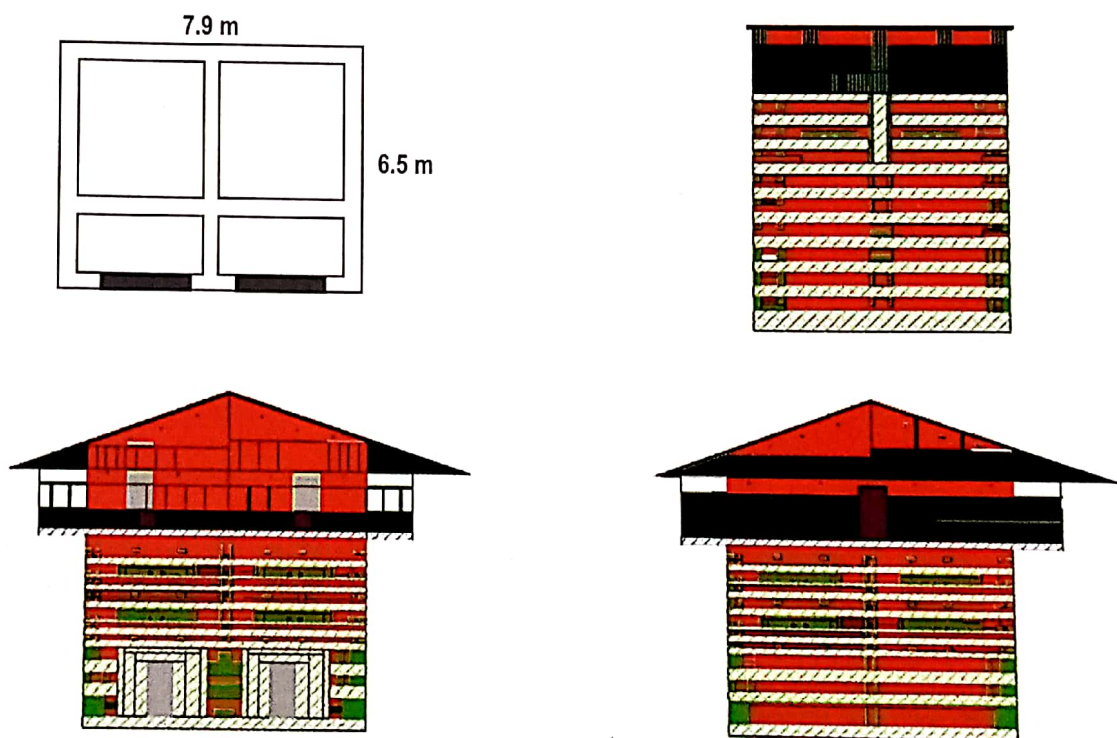
Fig.12: Plan, side, front and rear elevations of the Koti Banal structure.
