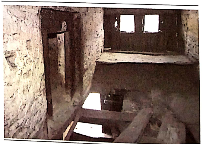
Fig.16: Internal wall with a door on the first floor. This wall lacks continuity from the ground floor.
