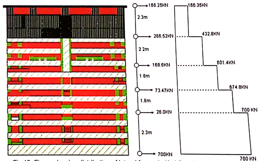
Fig.13: Figure showing distribution of lateral forces in Koti Banal structure
